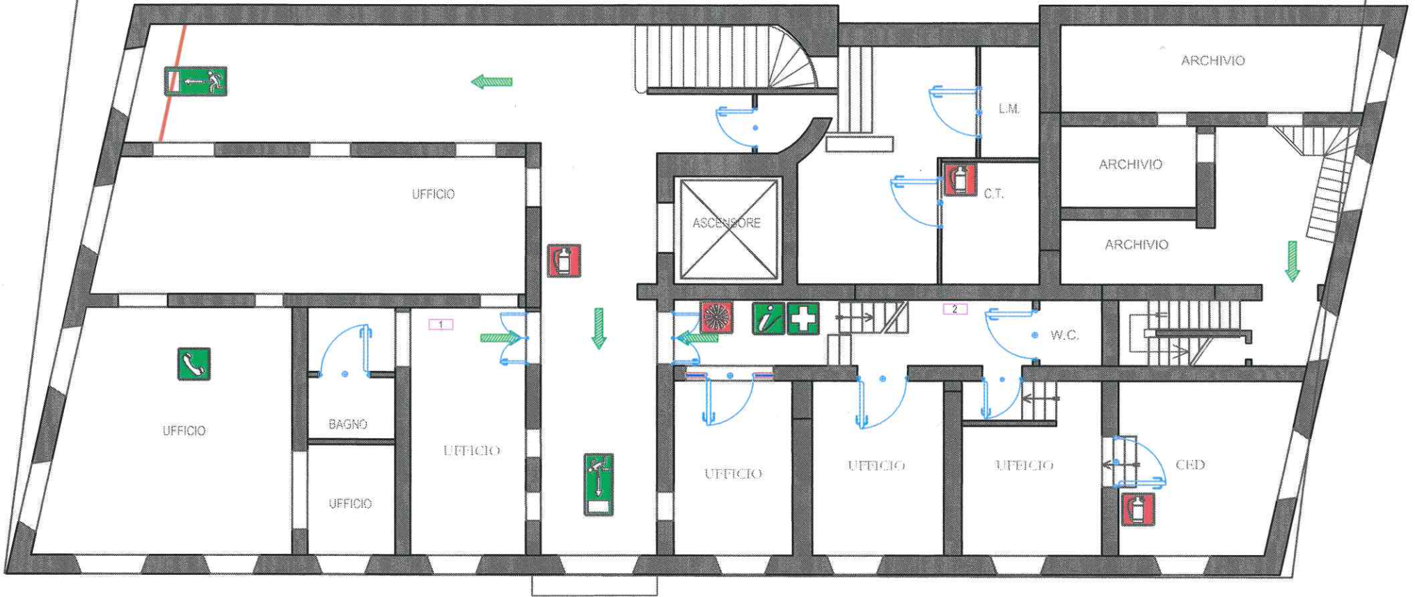
PIANO TERRENO
